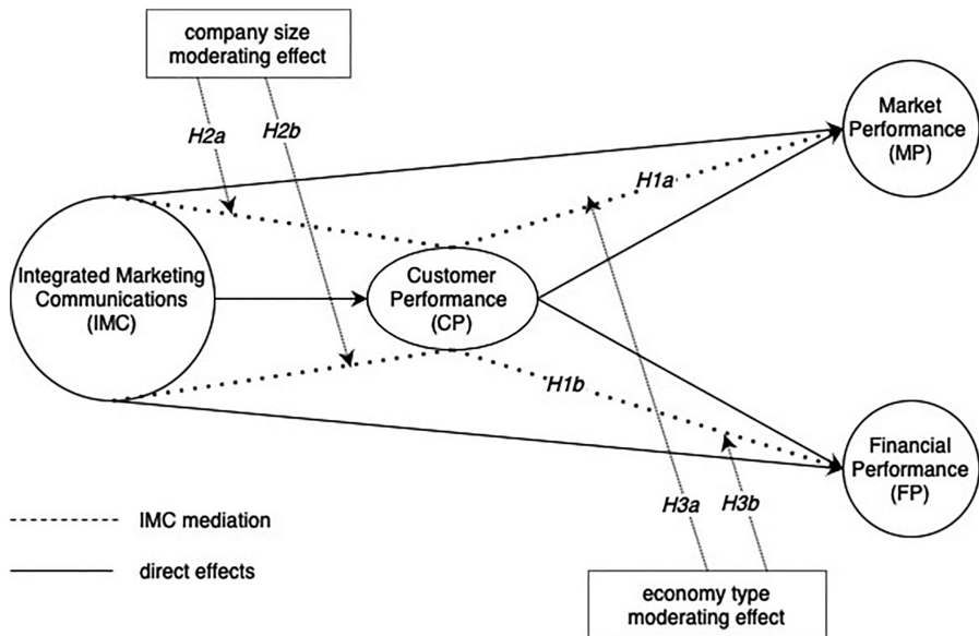
Figure 1. Hypotheses detail
